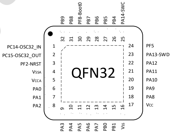
Figure3-5 QFN32(4*4) PY32F071K3xU7-E Pinout3 (Top view)
