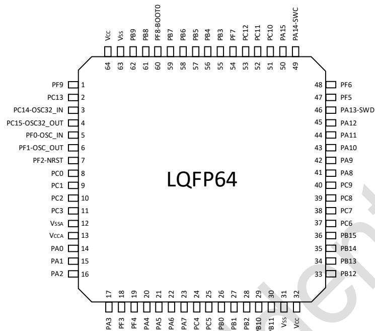
Figure 3-1 LQFP64 PY32F071R1xT7-E Pinout1 (Top view)
