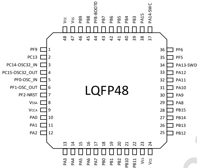
Figure3-3 LQFP48 PY32F071C1xT7-E Pinout1 (Top view)
