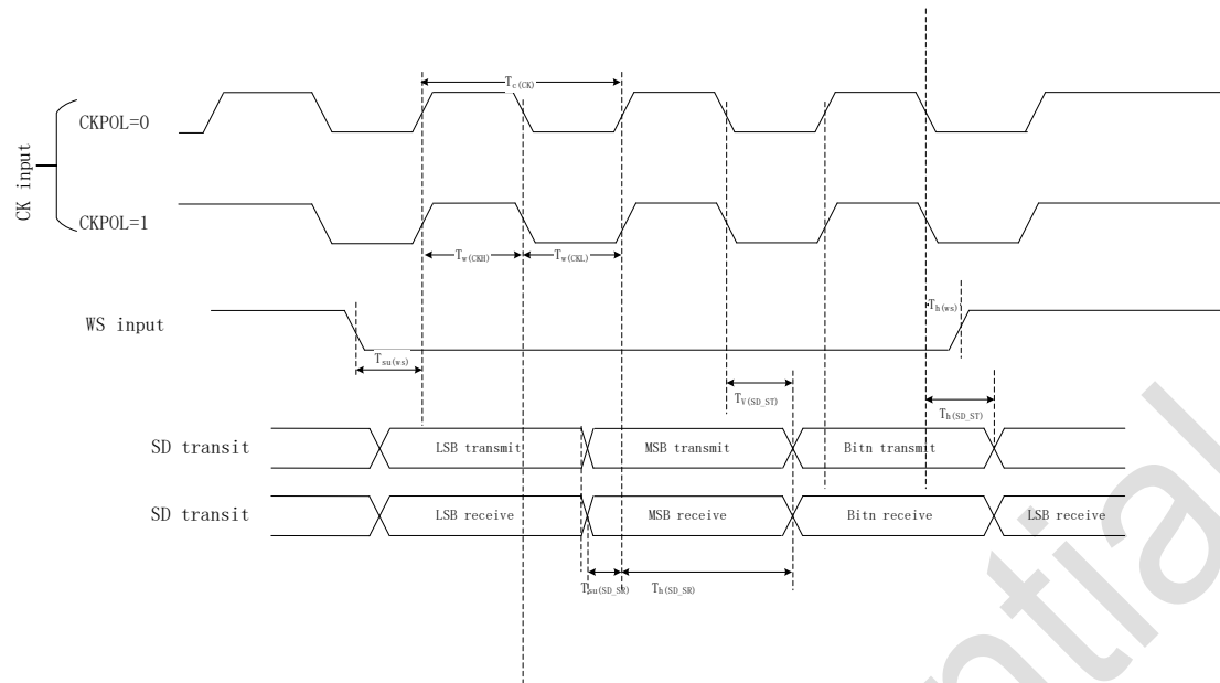
Figure 5-8 I²S timing diagram – Slave mode(Philips protocol)
