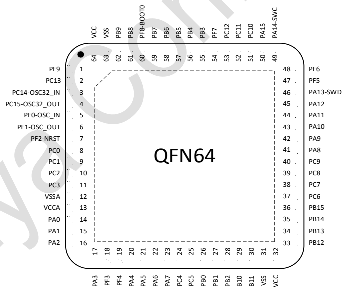
Figure 3-2 QFN64 PY32F071R1xU7-E Pinout1 (Top view)
