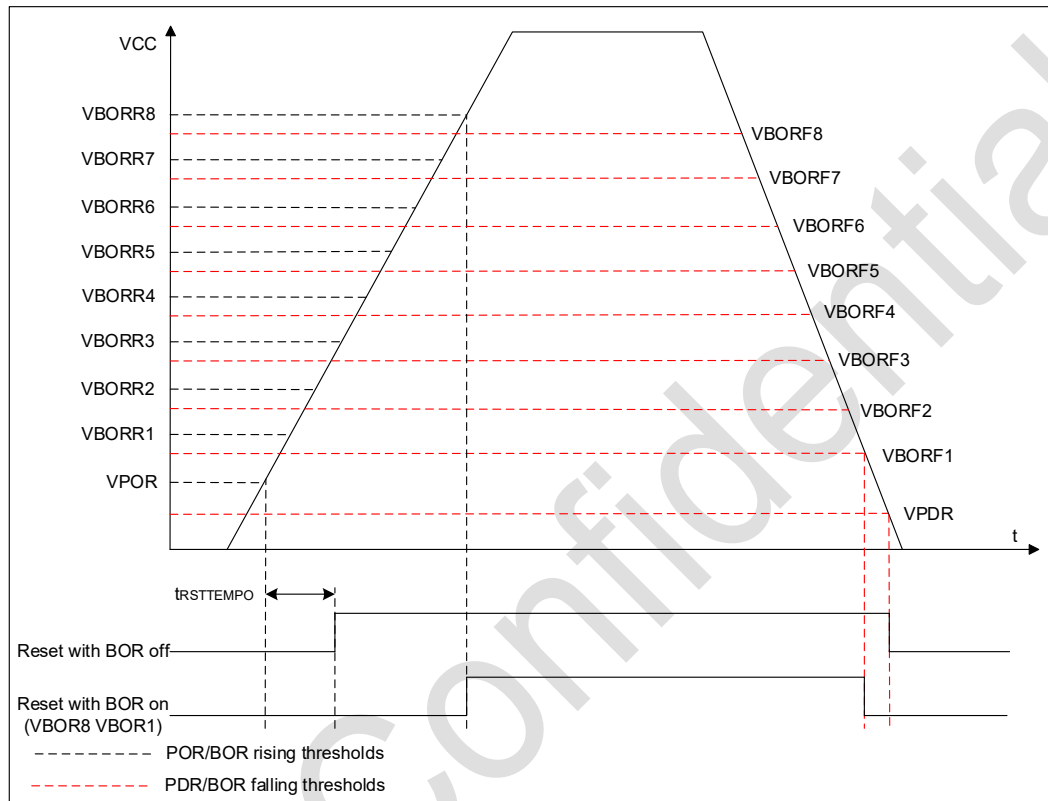
Figure 2-3 POR/PDR/BOR threshold
